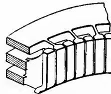
Fig. 5370. Perspective View of Segmental Chilling-blocks.
